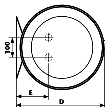
VERTICAL WALL-MOUNTED
