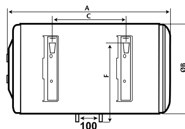
HORIZONTAL WALL-MOUNTED
