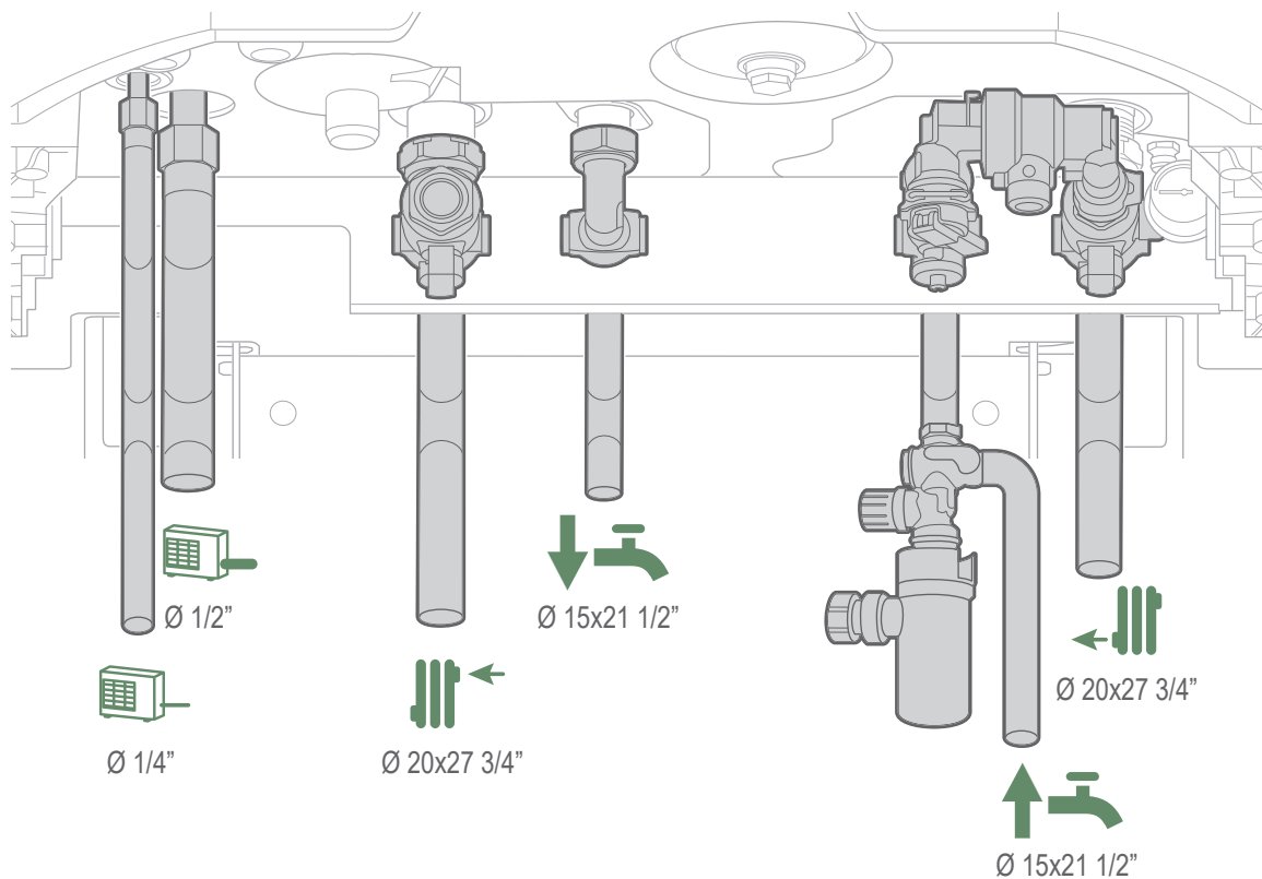
fig. 3 - Raccordements
