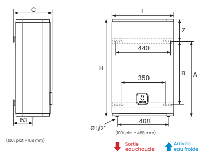
Vertical Mural 40 / 65 / 80 / 100L plat
