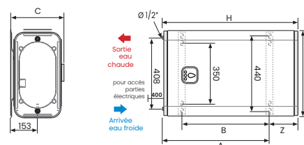
Horizontal Mural 40 / 65 / 80 / 100L plat
