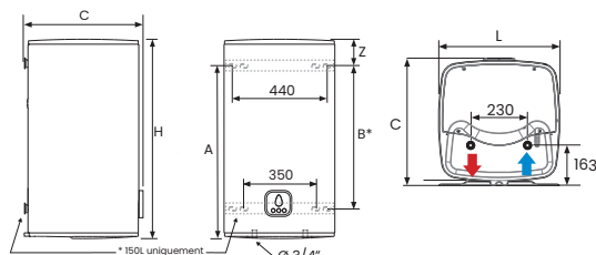
Vertical Mural 100 / 120 / 150L
