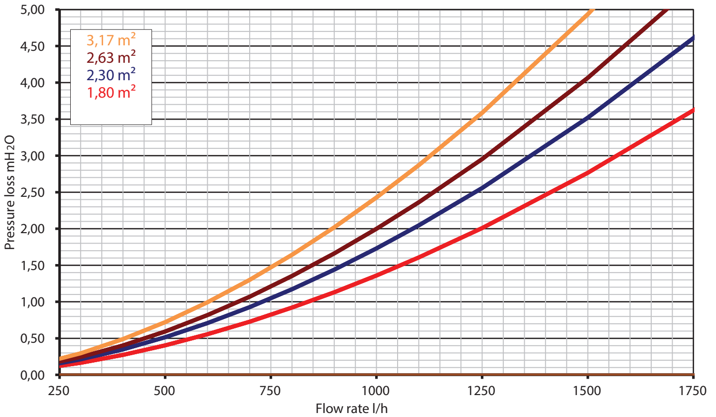
Pressure loss cooper coils single tubes (Water at 20 °C)
