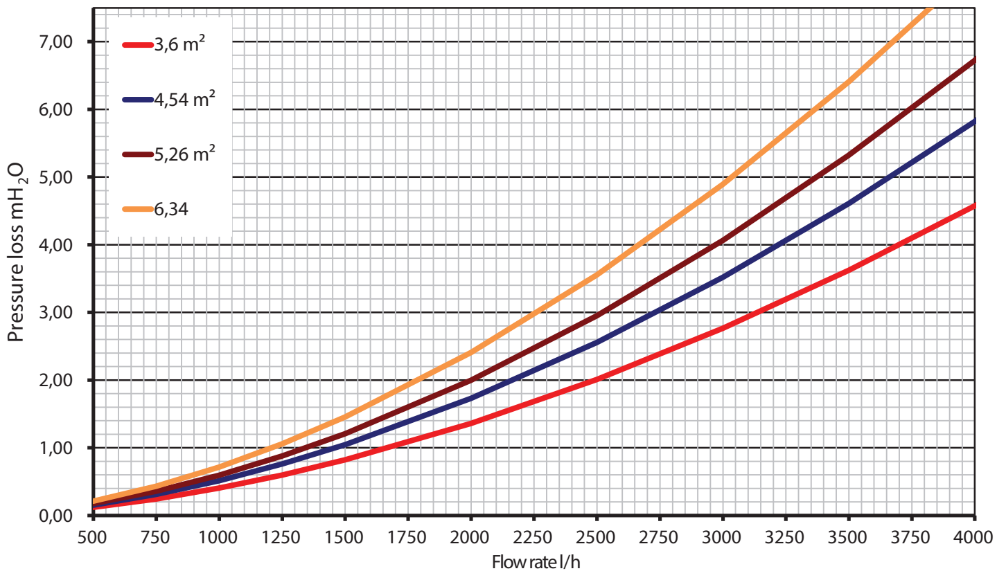
Pressure loss cooper coils double tubes (Water at 20 °C)
