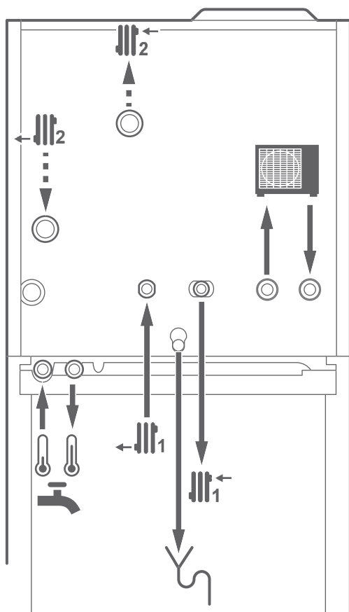
fig. 4 - Raccordements hydrauliques
