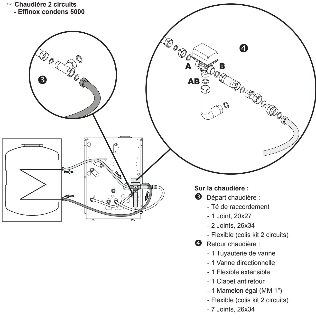
figure 9 - Chaudière 2 services
