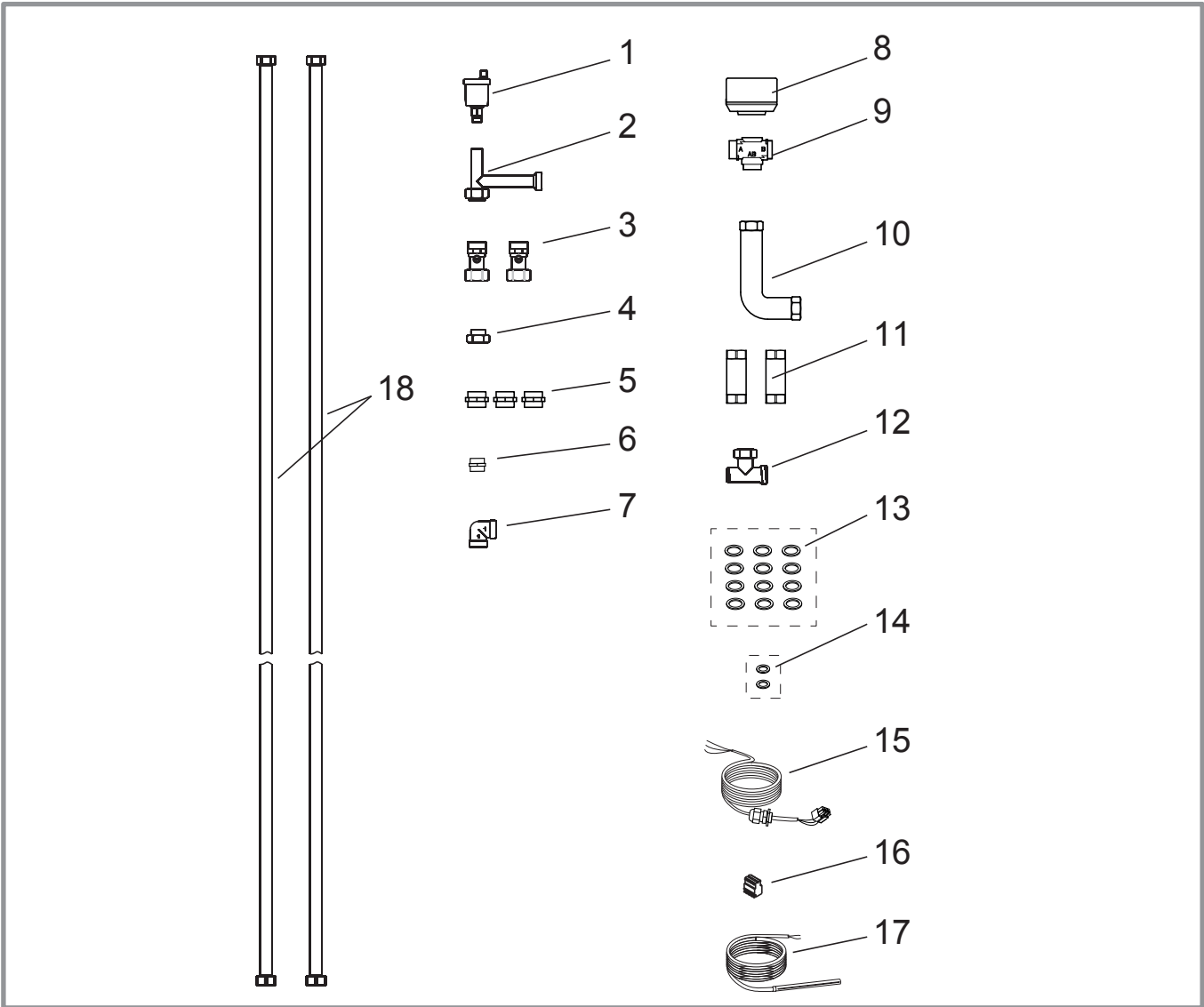
figure 13 - Kit de raccordement sanitaire
