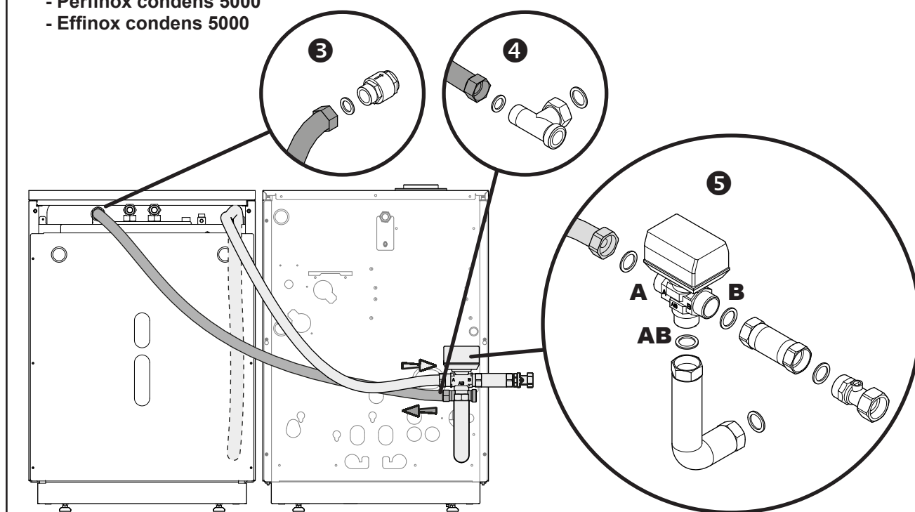
figure 8 - Ballon Sanit 100 et chaudière 1 service
