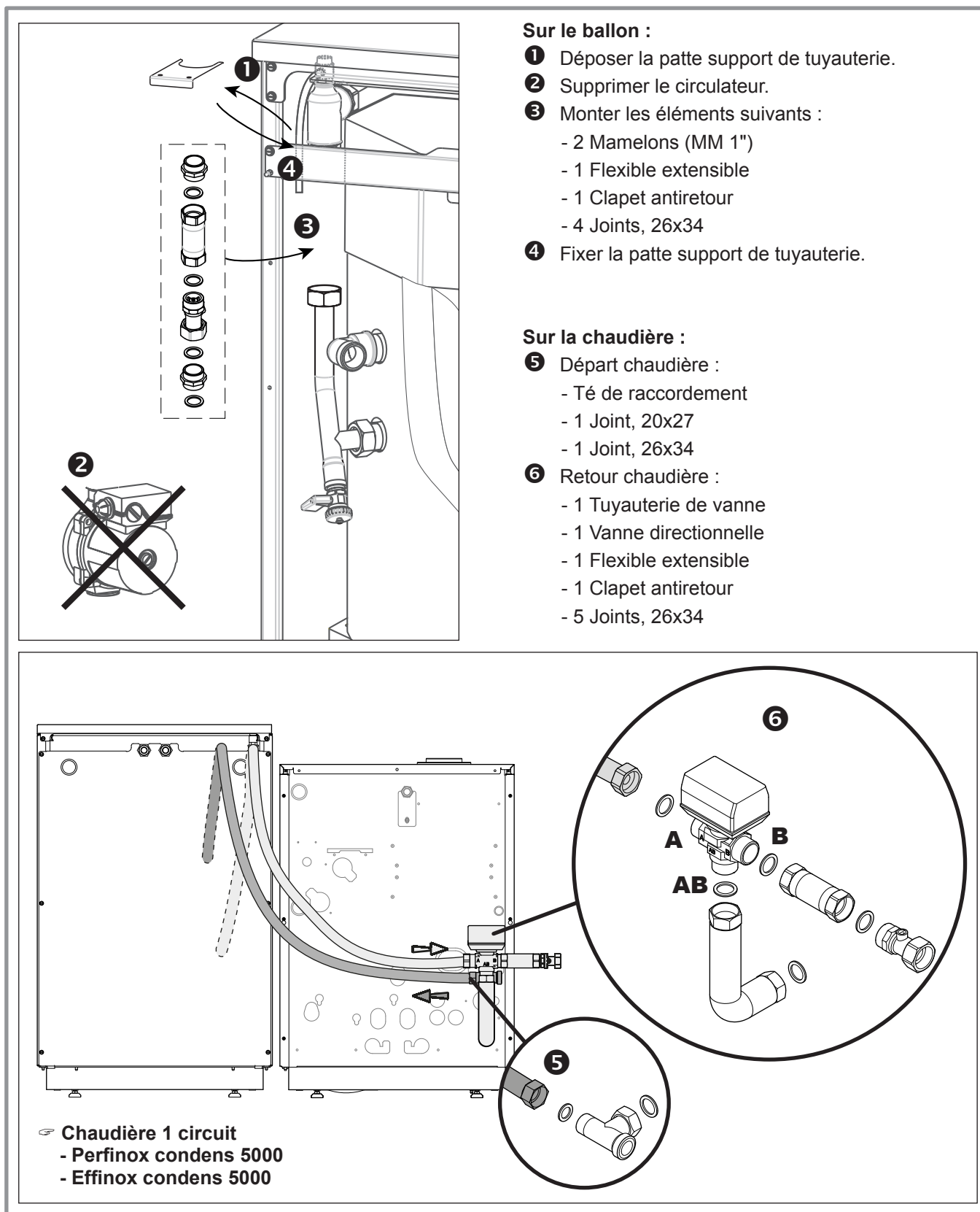
figure 10 - Ballon Sanit 105 / Sanit 130 et chaudière 1 service
