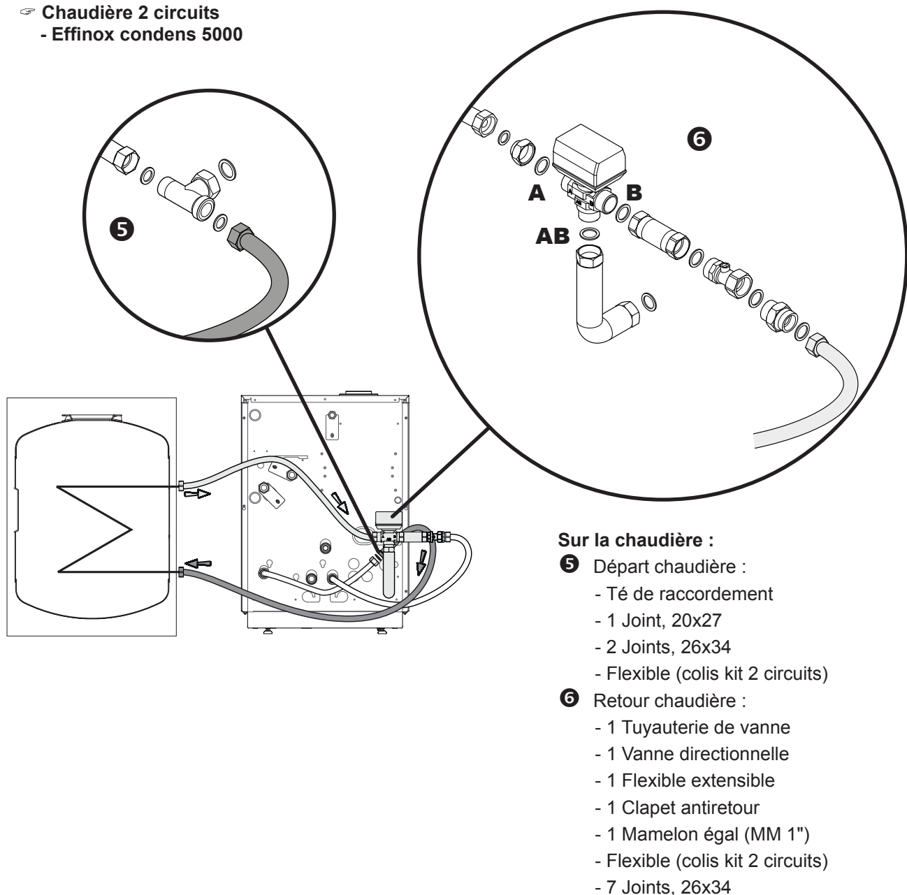
figure 11 - Chaudière 2 services
