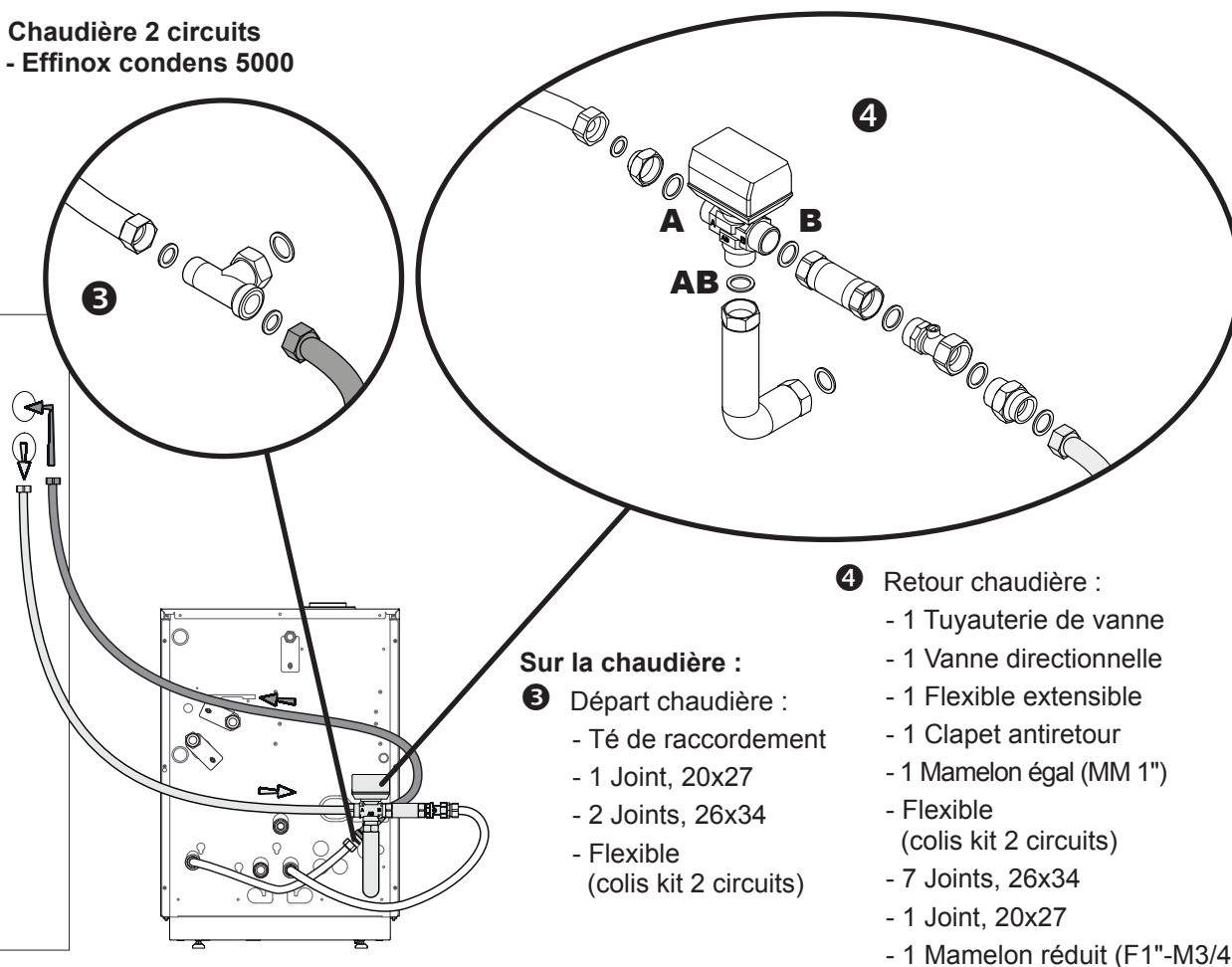
figure 7 - Chaudière 2 circuits
