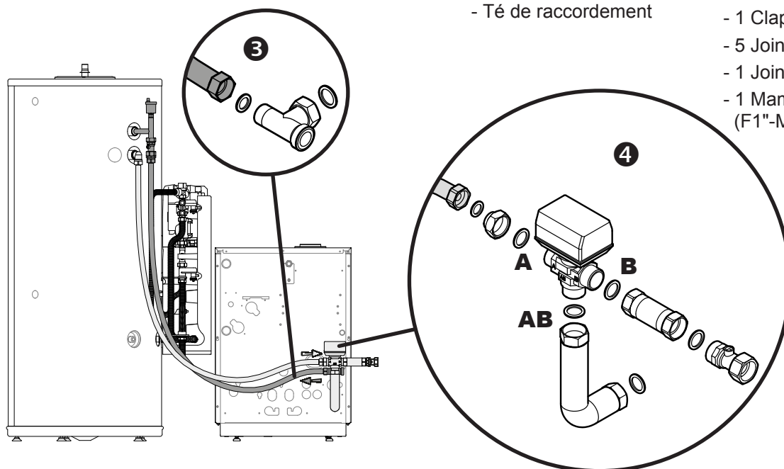
figure 6 - Chaudière 1 circuit
