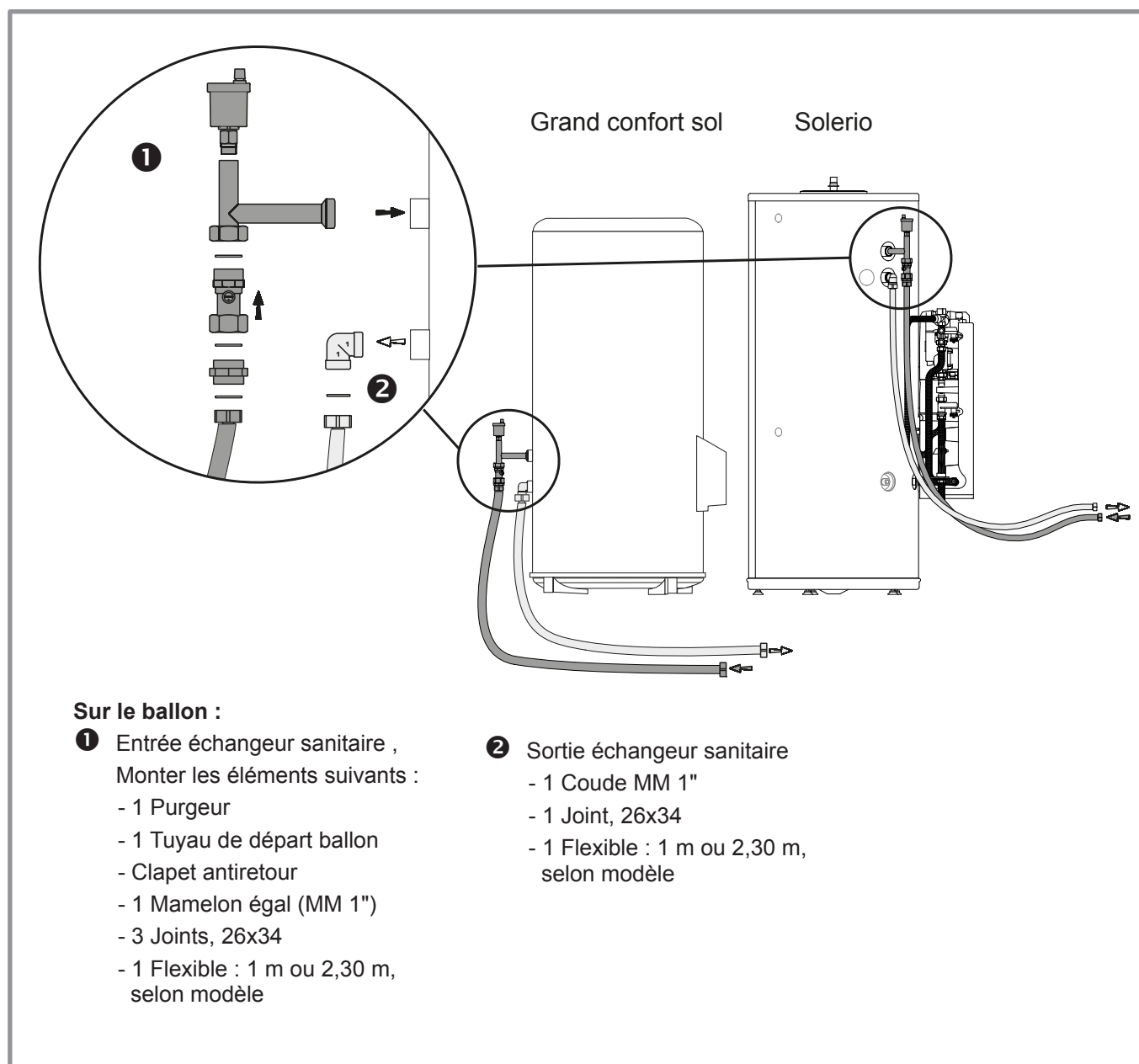
figure 5 - Ballons Grand confort ou Solerio
