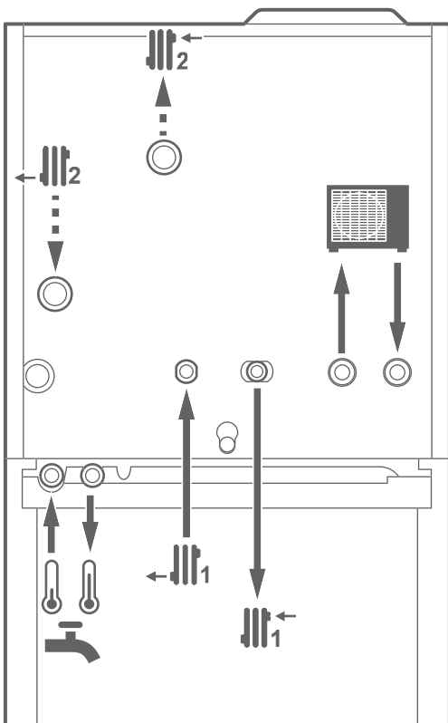
fig. 4 - Raccordements hydrauliques
