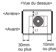
Fig. 2 Installation simple
