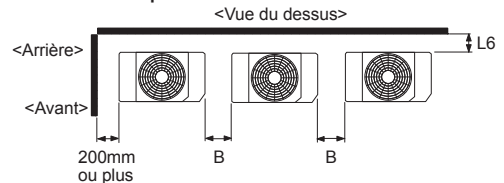
Fig. 9 Installations multiples
