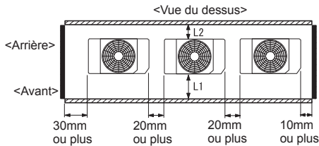
Fig. 3 Installations multiples
