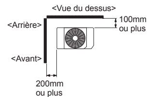
Fig. 9 Installations multiples
