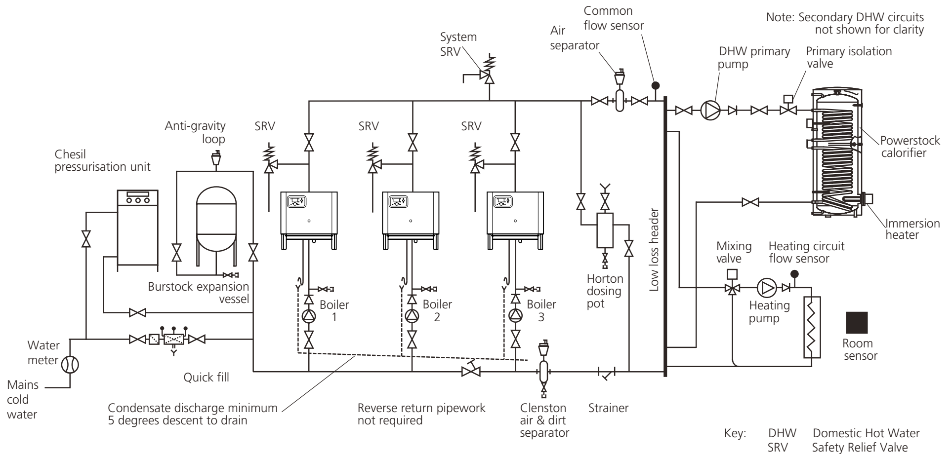
Scheme 3: Sealed system single pipe header, individual boiler pumps and low loss header
