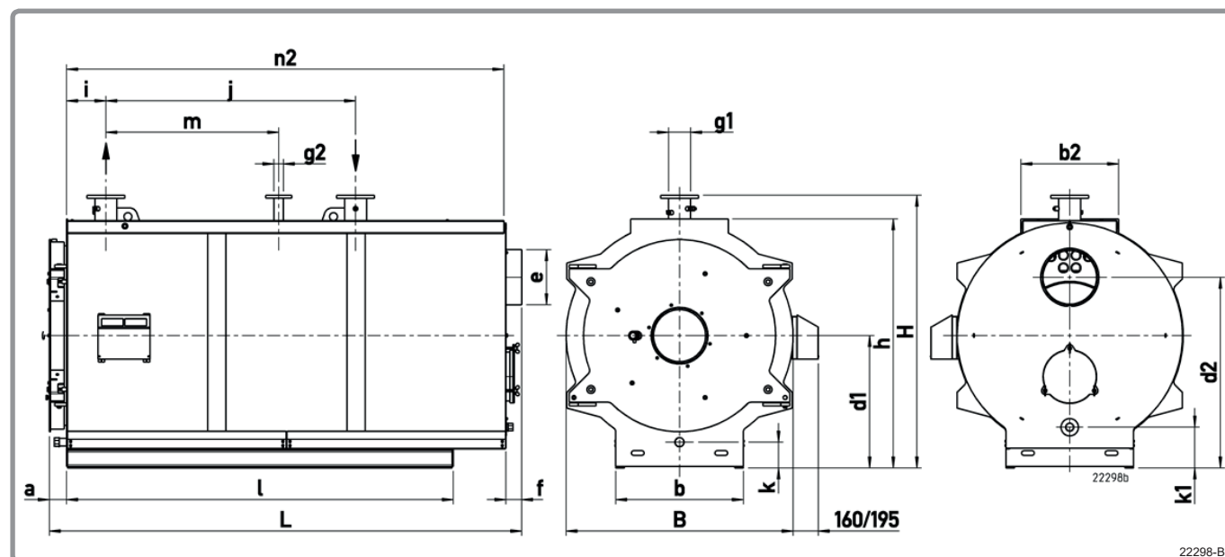
figura 2 - LRR / LRR-NT 47-52
