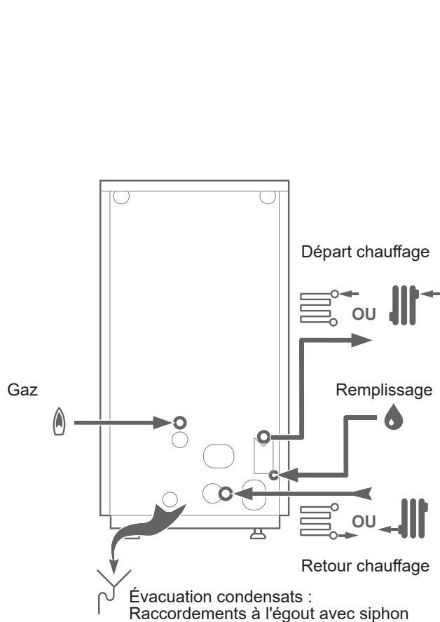
fig. 16 - Raccordements hydrauliques
