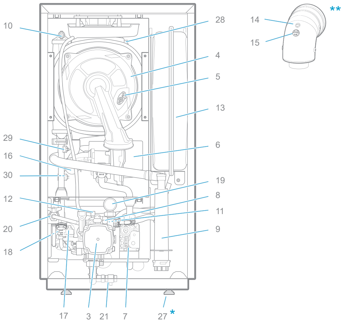
fig. 5 - Organes - Perfinox 2
