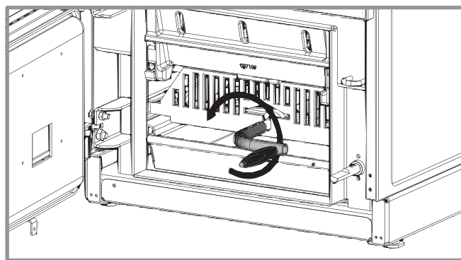
fig. 20 - Grille relevable
