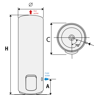
FLOOR-STANDING
