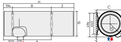
HORIZONTAL WALL-MOUNTED
