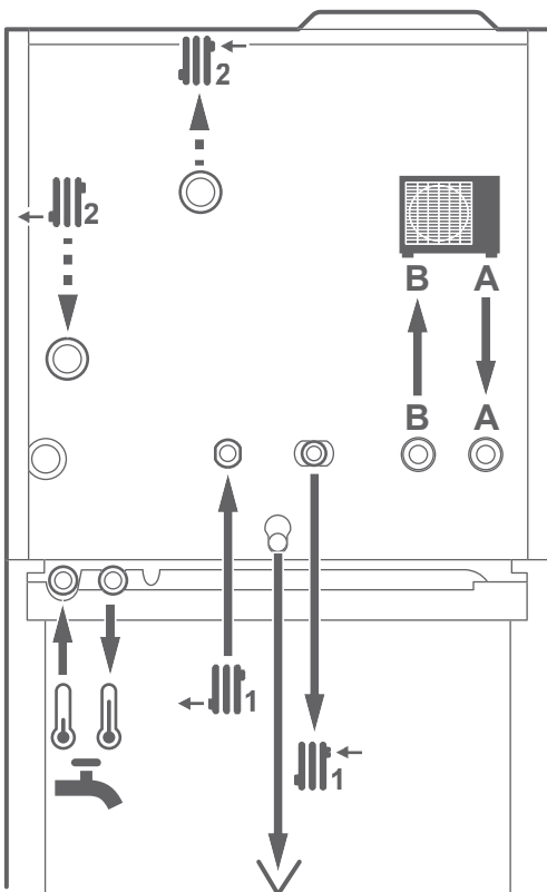
fig. 4 - Raccordements hydrauliques
