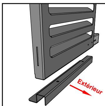
Fixation murale
