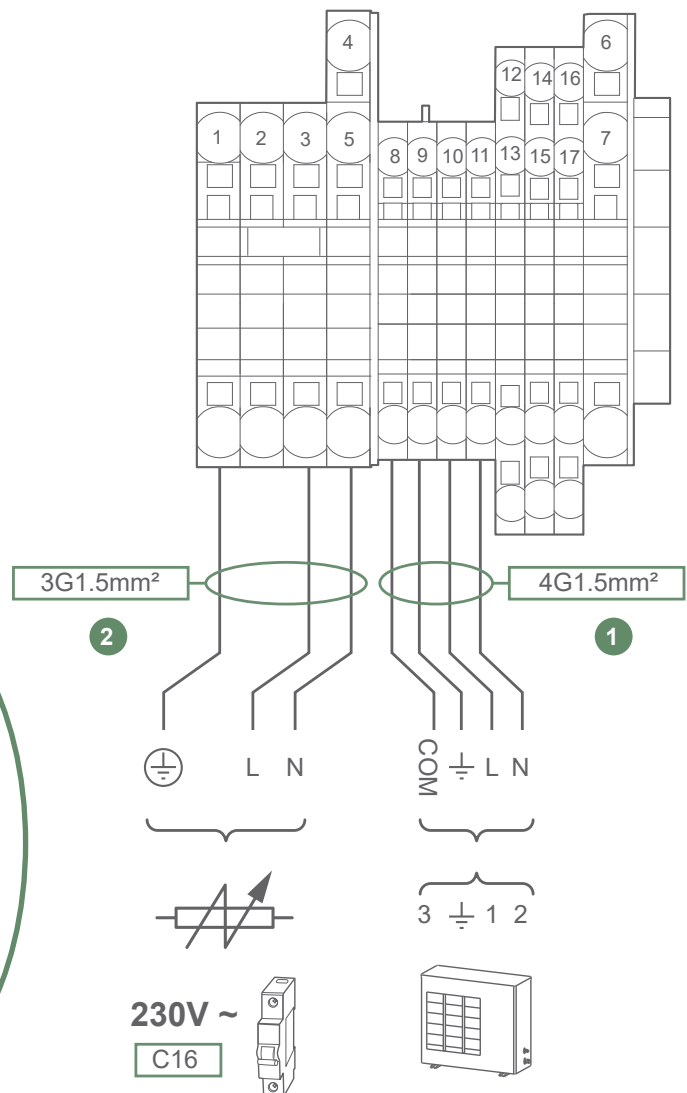
fig. 12 - Raccordements Alimentations
