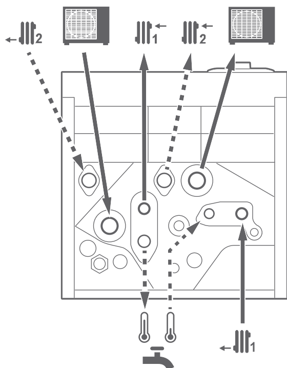
fig. 5 - Raccordements hydrauliques
