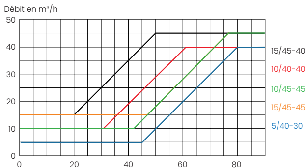
Bouche WC (BAW)
