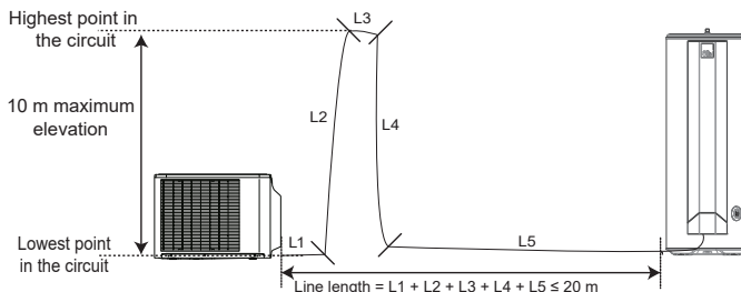
Installation example
