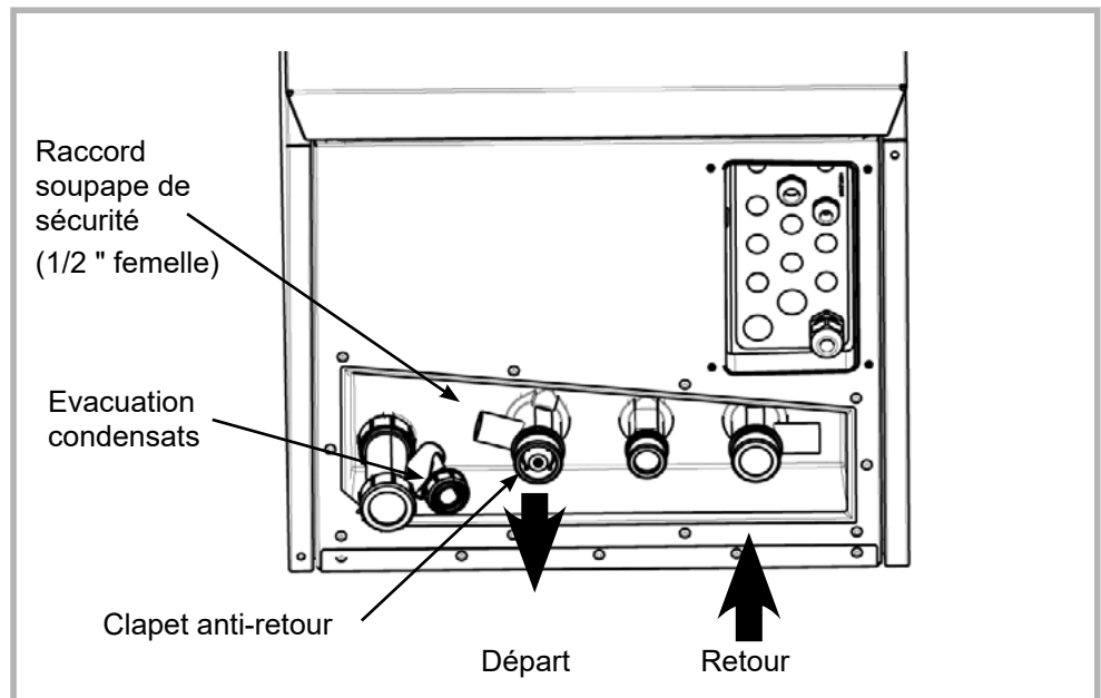
figure 21 - Eléments
