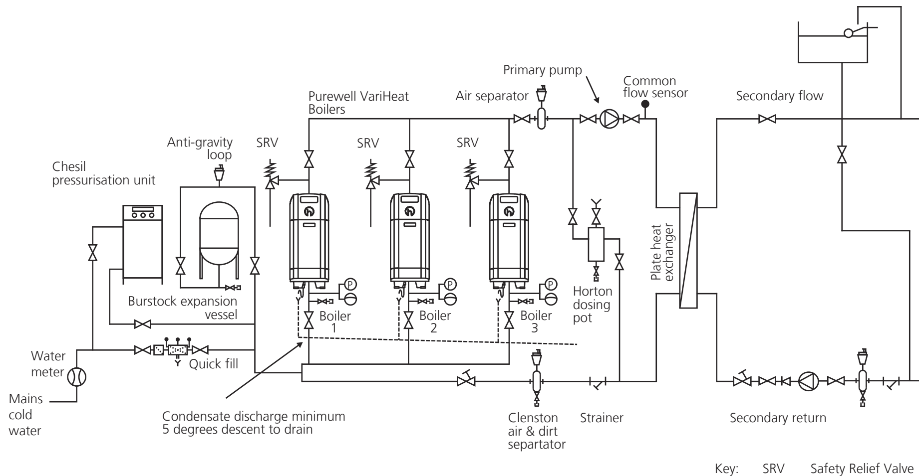
Purewell VariHeat c Scheme 3: Sealed Primary and Open Vented Secondary System with Plate Heat Exchanger Separation
